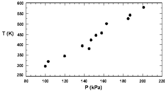
Figure A-1. Temperature versus pressure, as measured by the transducers.
